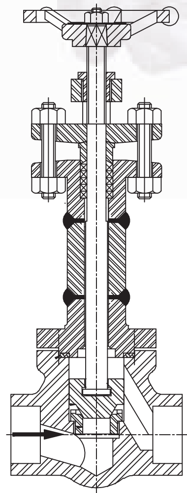
GLOBE VALVE
