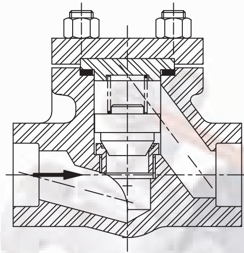
CHECK VALVE
